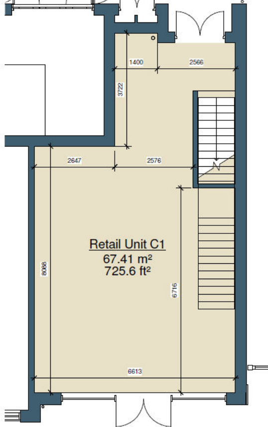
1 | C1 - Ground Floor Level 1 : 100
