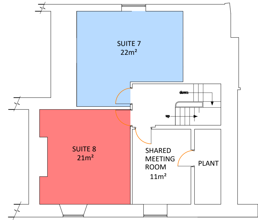
02 SECOND FLOOR PLAN 1:100
